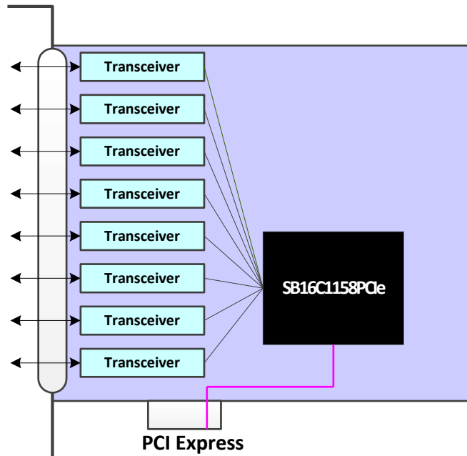
Figure 5-1: Serial 8-port Mode Application Block Diagram
